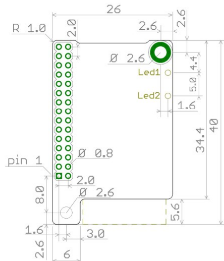
Horizontal mounting
